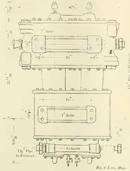
FIG. 3. NEW YORK DUPLEX AIR PUMP, No. 5.
